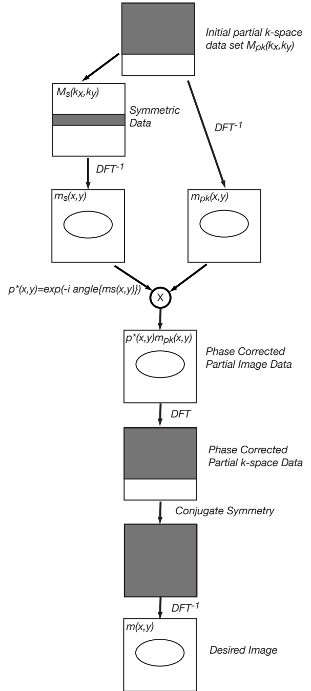
Figure 7: Summary of the phase correction and conjugate synthesis algorithm.
