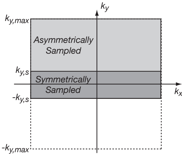
Figure 2: Partial k-space acquisition for reducing scan time by reducing the number of phase encodes required.
