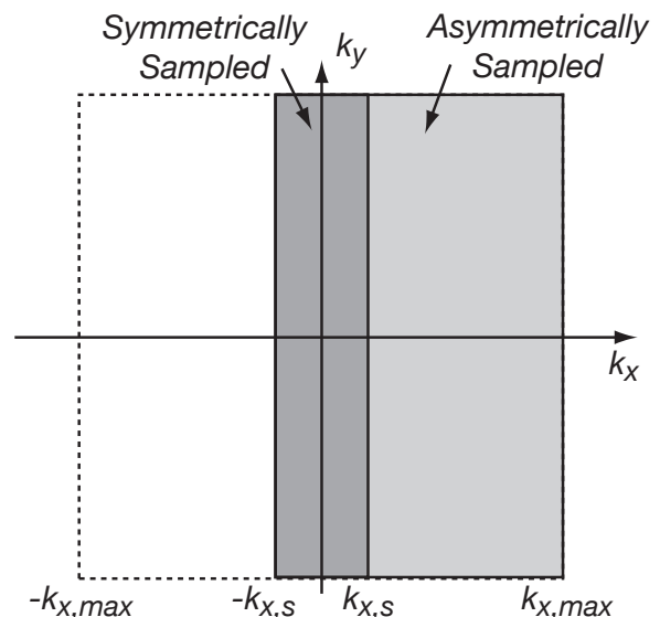
Figure 4: Partial k-space acquisition for reducing echo times by collecting only a fraction of the full echo.
