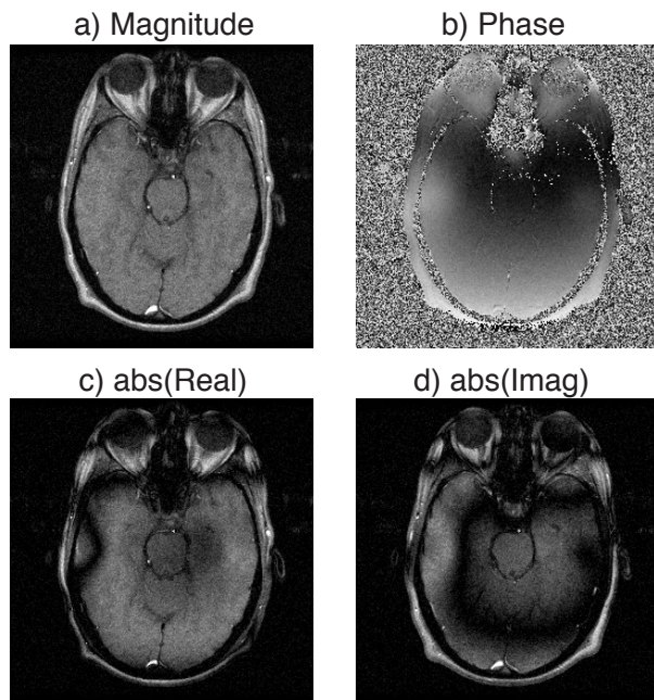
Figure 1: Axial gradient echo image acquired at 0.5T with an echo time of 13.8 ms. At this time water and fat are rephased. The linear shim terms have been corrected, leaving the non-linear components due to susceptibility shifts.
