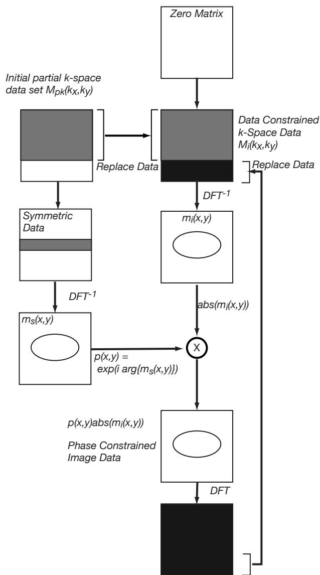
Figure 17: Summary of the POCS algorithm.
