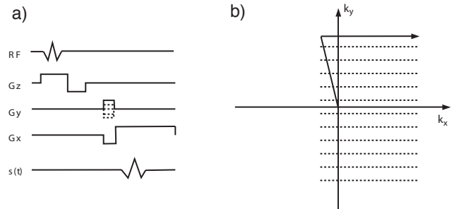
Figure 3: Pulse sequence with a reduced echo time, resulting in a partial echo readout.
