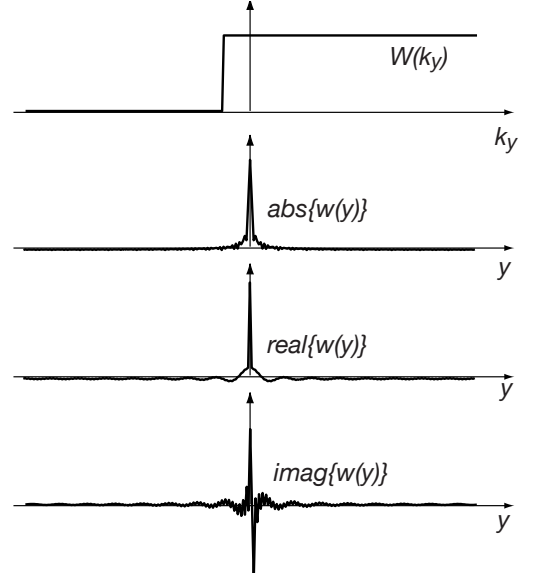
Figure 6: A k-space weighting function W(k_y) that truncates a full k-space data set into a partial k-space data set. In this case the k-space fraction is 9/16^{th} s, as in Fig. 5. The blurring evident in Fig. 5 is due to the convolution of the inverse transform of W(k_y) , which is plotted here in absolute value, and real and imaginary components.
