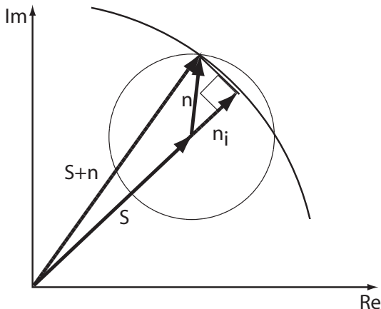
Figure 8: Magnitude operator suppression of the noise component that is in quadrature with the signal vector S . The magnitude of the sum |S + n| is approximately |S + n_i| , where n_i is the component of the noise that is in-phase with S .
