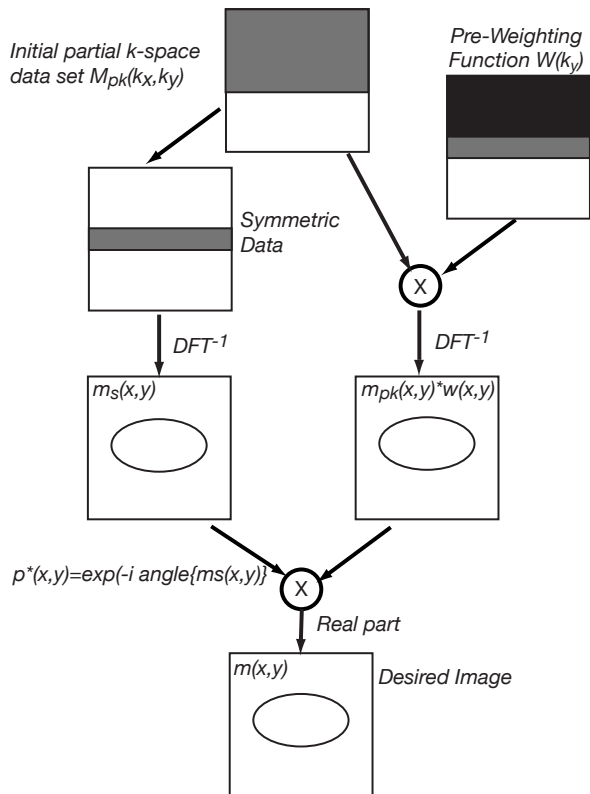
Figure 14: Summary of the homodyne algorithm.
