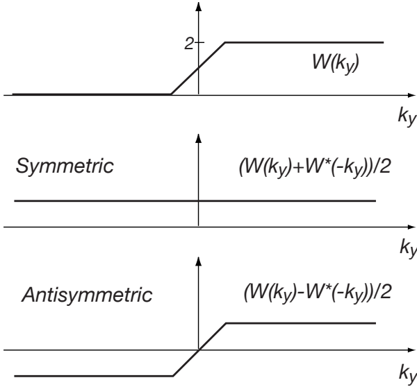
Figure 12: Using a linear ramp weighting over the central symmetrically sampled strip in k-space reduces the transients at the boundaries of the different k-space regions, and still produces a uniform k-space weighting for what will be the real component of the image.
